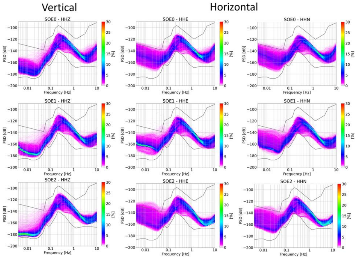
Fig.4. Probabilistic power spectral densities (PPSD) of the vertical and horizontal channels from surface (SOE0) and underground stations (SOE1, -84m, and SOE2, -111m) during the first half of 2021. For comparison also the Peterson's model curves (NLNM, new low noise model, and NHNM, new high noise model) are drawn. SOE0 and SOE2 are operated without amplification, with the standard input range of 40Vpp at the digitizers, while SOE1 is operated with the reduced input range of 4Vpp: in this case the improvement in the measure can be observed from 3Hz to 10Hz, indeed in this band the digitiser self-noise sets a limit to the measured noise in the other stations operated with standard settings.
