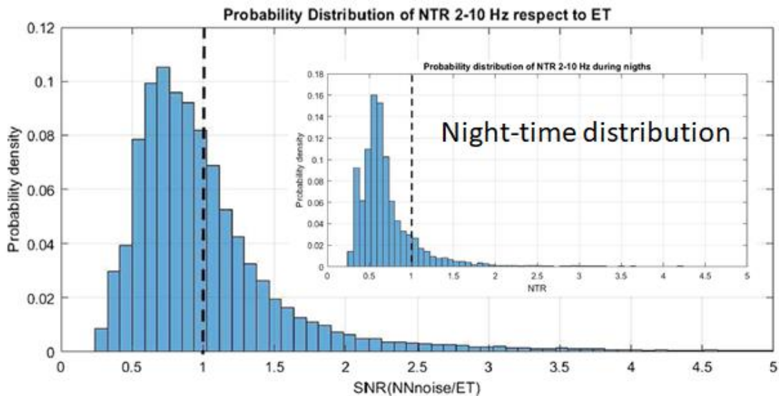
Fig.26. Noise-to-target ratio (NTR) probability distribution over the whole period [4].
