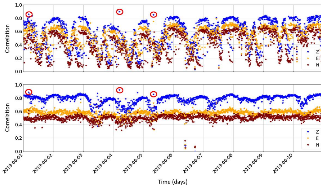
Fig.13. Correlation between seismic stations versus time for nine days of June 2019 in the band 1\text{Hz} < f < 10\text{Hz} for all the three channels (vertical and horizontals) [3]. In the top panel the correlation between SOE0 (surface) and SOE2 (underground) is shown, the night-day pattern is evident. In the bottom panel the correlation between SOE1 and SOE2 (both underground) is shown, in this case with a mild night-day pattern only in the vertical channel. Red circles indicate three earthquake detections.
