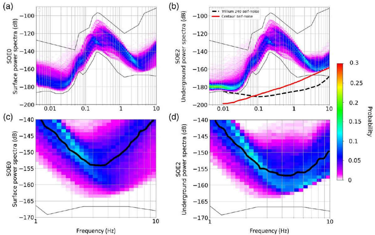
Fig.3. Probabilistic power spectral densities (PPSD) of the vertical channels from surface (SOE0 station) and -111m underground (SOE2 station) during the 2020 [3]. For comparison also the Peterson's model curves (NLNM, new low noise model, and NHNM, new high noise model) are drawn. Note that both stations are operated without amplification, with the standard input range of 40Vpp at the digitizers.
