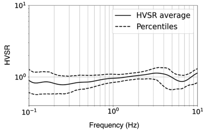
Fig.9. Average horizontal-to-vertical ratio (HVSr) of SOE0 in the period 1 January - 30 April 2020 [3]. Dashed lines are the 5th and 95th percentiles.
