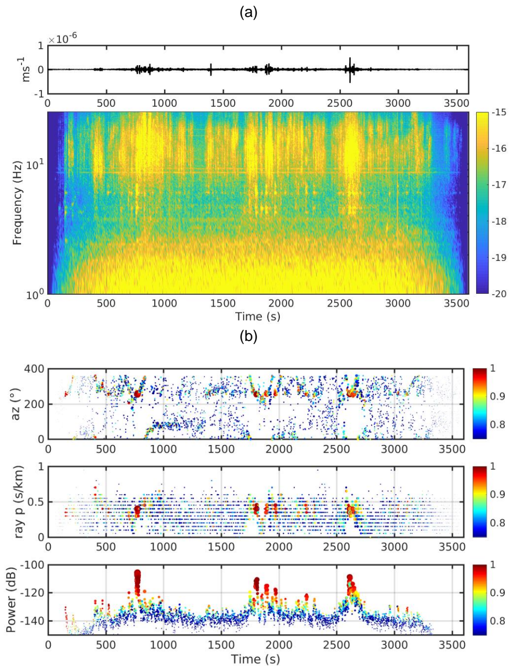
Fig. 21 - (a) Sample vertical-component recording of ground velocity at array station A01 (top). Data are band-pass filtered over the 1-25 Hz frequency band to better highlight the contribution of cultural noise. At the bottom, the array-averaged distribution of spectral power as a function of time and frequency (spectrogram) of the same signal. Colors indicate the \log_{10} of power, according to the color bar at the right. (b) Results from slowness analyses for the sample frequency of 6.0 Hz. From top to bottom, the panels report the propagation azimuth (measured clockwise from N), the ray parameter, and the power of the slowness spectrum. Symbols are sized according to the RMS amplitude of the signal, and colored according to the multichannel coherency (color bars at the right). The analyzed time interval has length 1 hour, and begins at 05:33:20 UTC on January 21, 2021.
