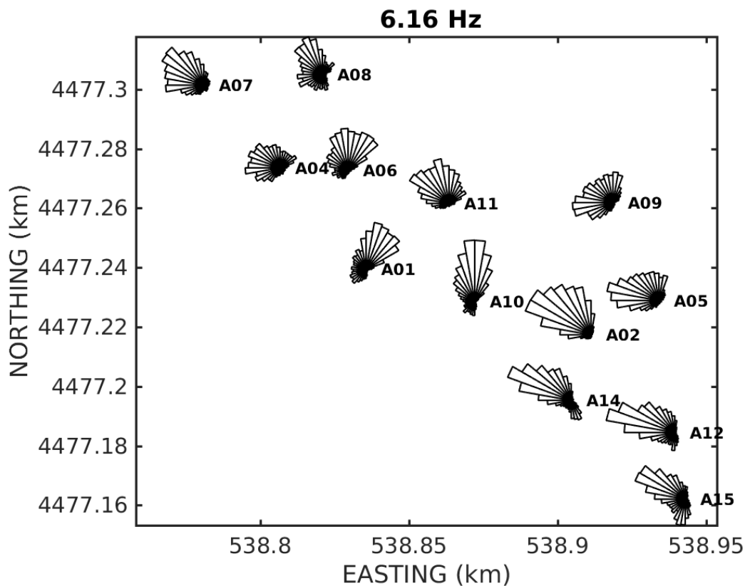
Fig. 24. Distribution of the polarization azimuths at the different array elements, for a fixed reference frequency.
