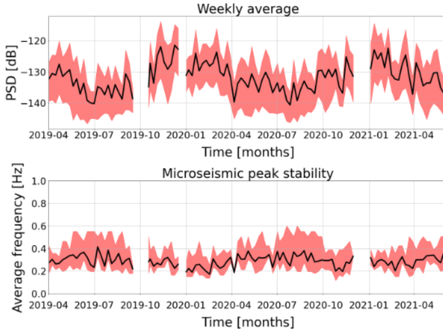
Fig.15. Microseismic trend (PSD at 4.5s) observed at Sos Enattos in the period 2019-2021 and frequency peak stability [5,6].
