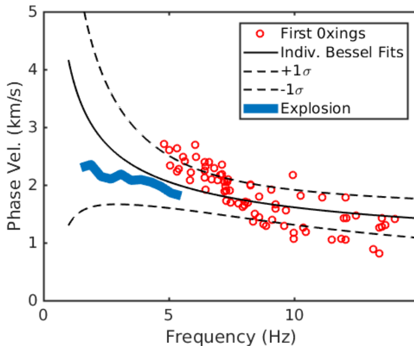
Fig. 19. Phase velocities derived from the first zero-crossing of the correlation functions (red circles), and through fitting individual correlation functions using power-law dispersions (black line). The blue stripe indicates the dispersion relationship obtained from analysis of mine blasting recordings (see Fig. 12).
