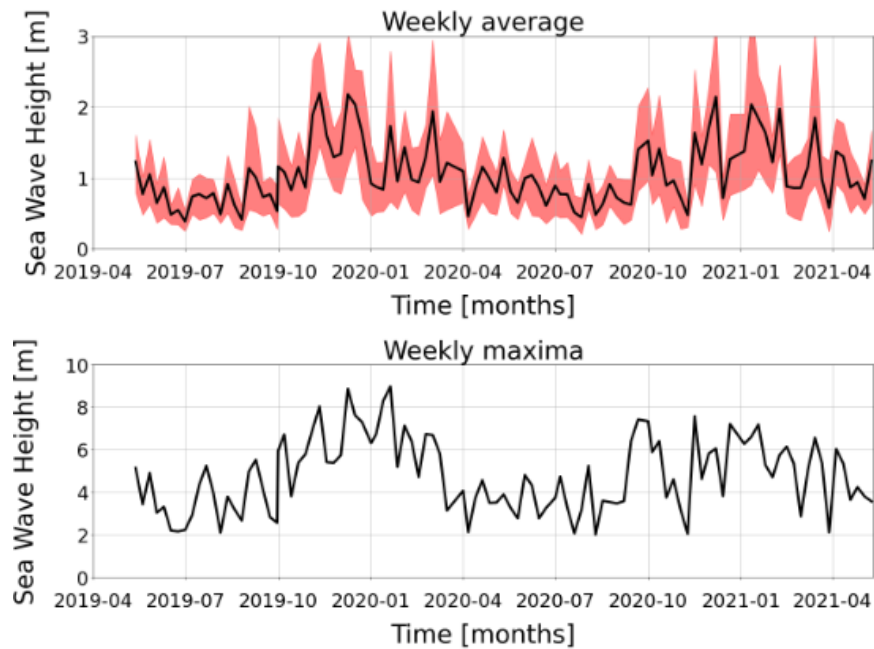
Fig.16. Weekly microseismic trend compared with the sea wave height in the period 2019-2021 [5,6].
