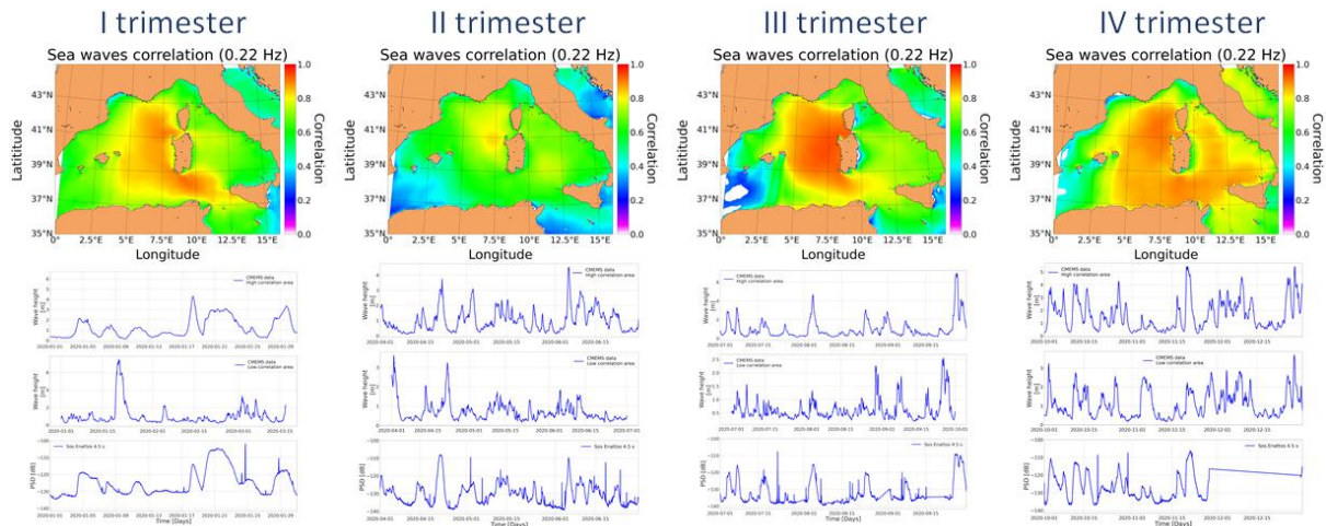
Fig.14. Correlation between the average sea wave height from CMEMS and the seismic noise at Sos Enattos in 2020, each panel indicate a trimester, with the top sub panel showing the correlation in the Mediterranean sea around the island of Sardinia, and the low sub panel showing the wave height respectively for high and low correlation areas and the seismic PSD at 4.5s observed at Sos Enattos.
