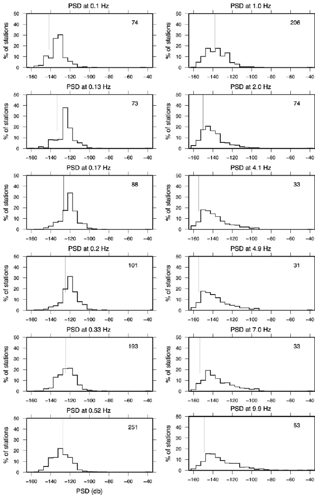
Fig.7. Ranking of the SOE2 station among the 445 stations of the Incorporated Research Institutions for Seismology virtual network FDSN+ALL in the period January-March 2020 [3]. For each frequency bin (indicated at the top of the panels) we calculate the mean PSD (in dB). The vertical bars indicate the average level of noise observed in SOE2 in the same time span, while the numbers indicate the ranking with respect to the selected global network.
