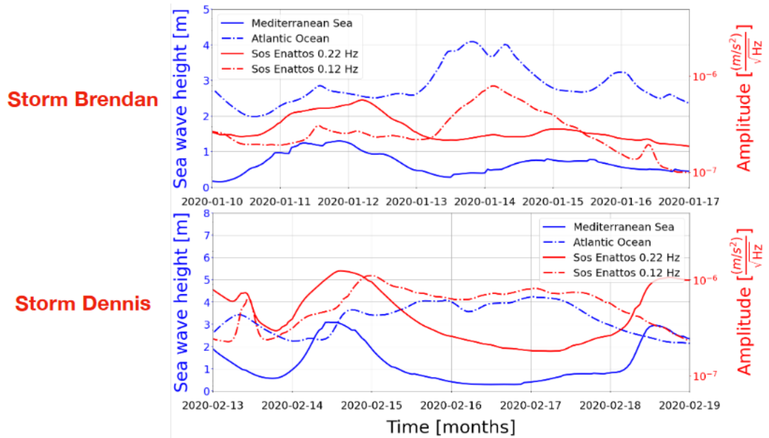
Fig.17. The effect of the sea wave during the Atlantic storms Brendan and Dennis on the microseismic peak [5,6]
