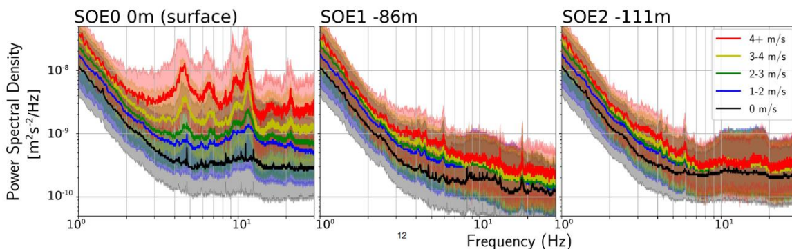
Fig.10. Seismic noise background measured in coincidence with a given wind speed at surface in the three stations SOE0, SOE1 and SOE2. Spectra are calculated over one minute following the wind speed measurement every 30 minutes [5,6].
