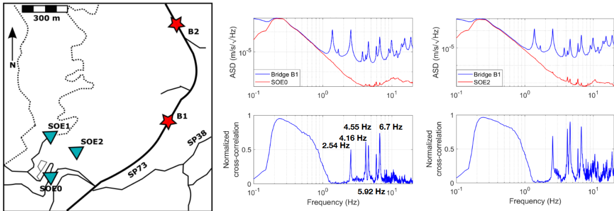
Fig.11. Left panel: map of the relative locations of Sos Enattos seismic stations and the nearby bridges (B1 and B2) along the SP73 road. Center and right panels: ASD of seismic background measured by geophones below the B1 bridge pillars (blue) compared to the seismic background (red) at SOE0 (center panel) and SOE2 (right panel); the cross-correlation between them is shown at the bottom of the panels.
