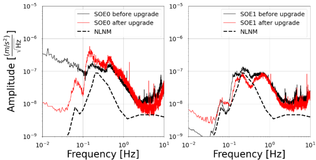
Fig.2. Data quality improvement in stations SOE0 (left) and SOE1 (right) provided by the sensor replacement (SOE0) and reduction of the input range (SOE1) [5].
