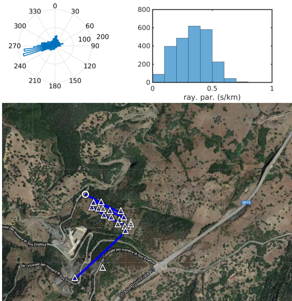
Fig. 22 - Top left: Rose diagram indicating the prominent directions of propagation derived from the slowness results shown in Figure 21. Only data associated with a coherency larger than 0.75 are considered. Top right: Distribution of ray parameters for the same time interval. Bottom: Enlarged map view of the array and surroundings. The observed directions of propagation suggest that most of the noise at frequency \sim 6\text{Hz} is associated with a bridge on Provincial Route SP73, visible at the right margin of the map.
