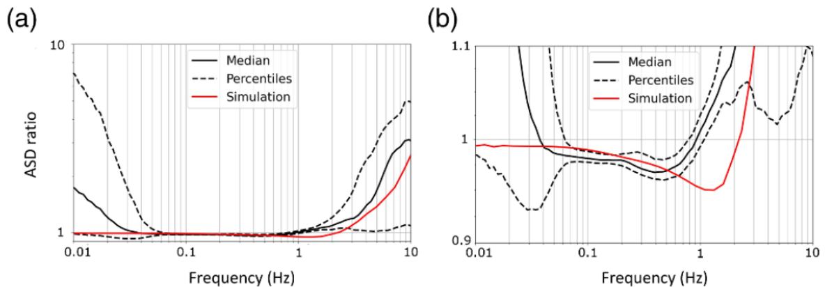
Fig.8. (a) Vertical component SOE0/SOE2 amplitude spectral density (ASD) ratio (median, black line) and 5th and 95th percentiles (dashed lines) compared with the corresponding amplitude ratios estimated from synthetic seismograms (red line) [3]. (b) Zoom around ASD=1 .
