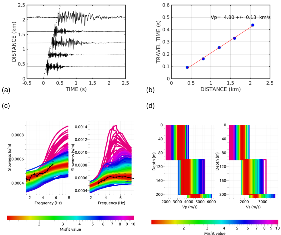
Figure 11. (a) Recordings of the vertical component of ground velocity associated with the blasting fired at 8:36:10 UTC on 18 October 2018. Traces are individually normalized to their maximum amplitude. (b) Apparent P-wave propagation velocity derived from the linear fit of P-wave arrival times as a function of the distance from the source. (c) Phase- (left panel) and group- (right panel) velocities measured over the [2,5.5] Hz and [3,8] Hz frequency intervals, respectively. The measured dispersion data are indicated by black dotted lines, and are compared to the predictions from the ensemble of investigated velocity models (colored patches). (d) Compressional- (left panel) and shear- (right panel) waves velocity models derived from the joint inversion of the phase- and group-velocity dispersions shown in (c). Colors in (c,d) correspond to the inversion misfit, according to the color bars at the bottom.
