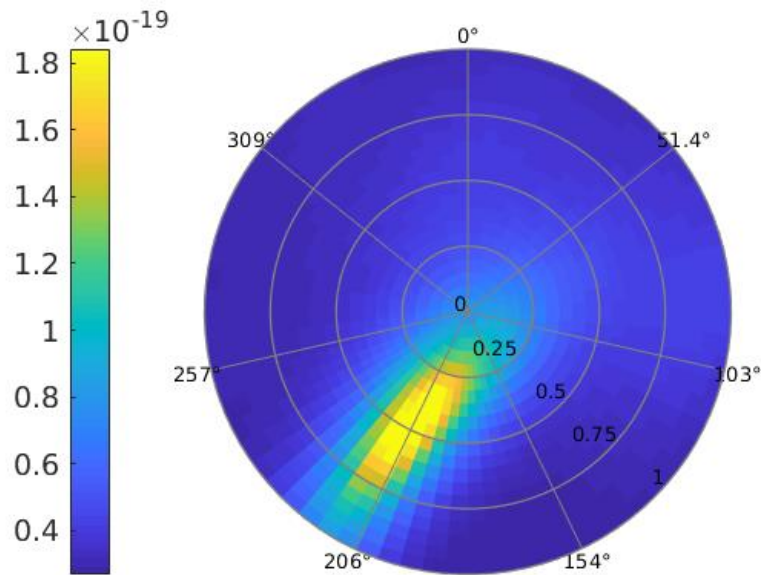
Fig. 20. Sample slowness power spectrum calculated over the 7-11Hz frequency band. The position of the spectral peak corresponds to a plane wave propagating with a ray parameter around 0.5 \text{ s km}^{-1} (i.e., an apparent velocity of about 2 \text{ km s}^{-1} ), toward a direction \sim 210^\circ\text{N} . The source is therefore located \sim 30^\circ\text{N} of the array.
